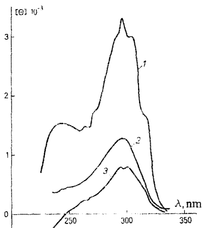
Fig. 1. Circular dichroism curves in heptane: 1) optically pure piperidone diastereomer Va, 2) 1:1 mixture of diastereomers V and Vb, 3) 28:72 mixture of diastereomers Va and Vb.
